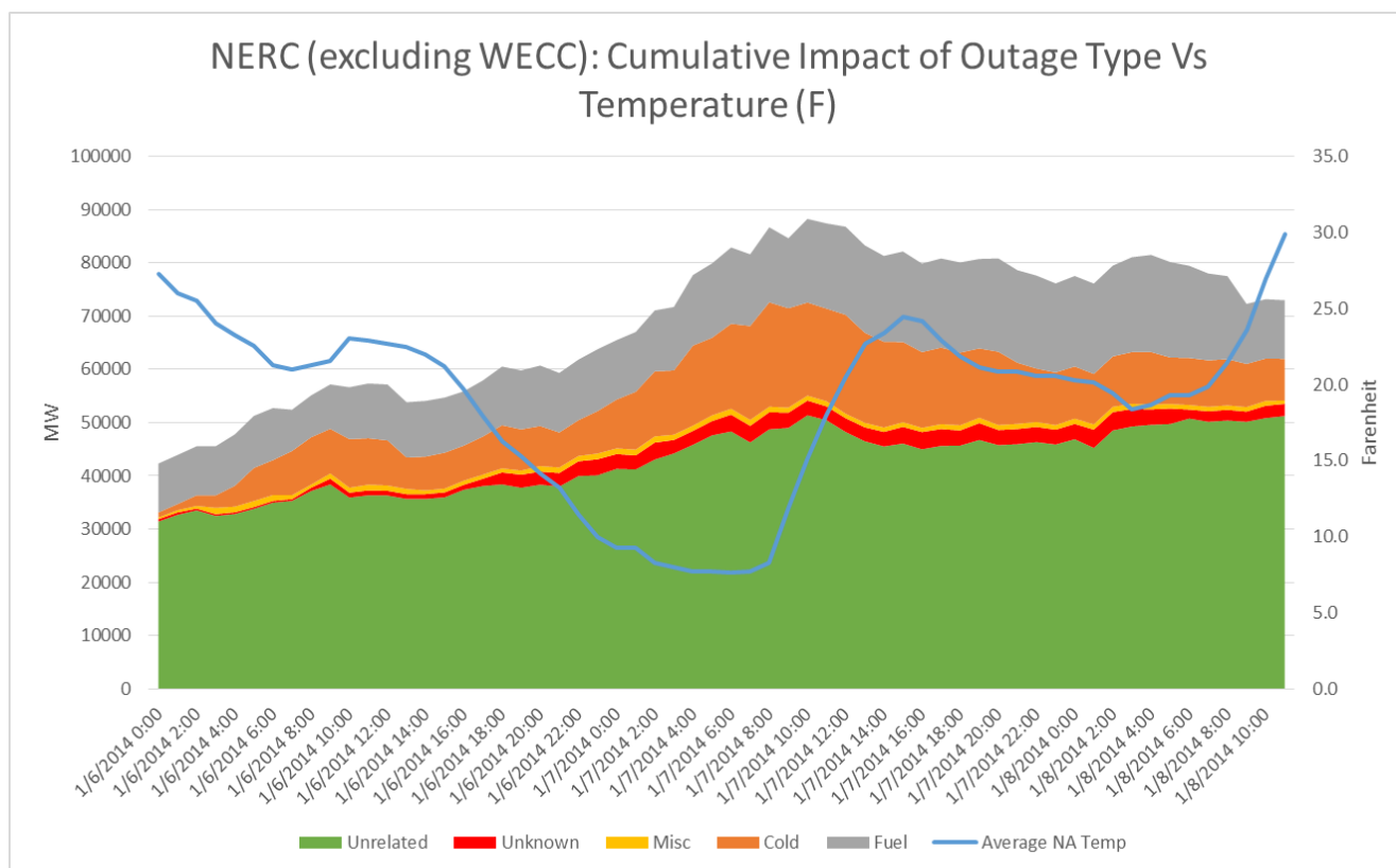
Figure 5: Total Outages in the Eastern Interconnection and ERCOT by Outage Type vs. Temperature
